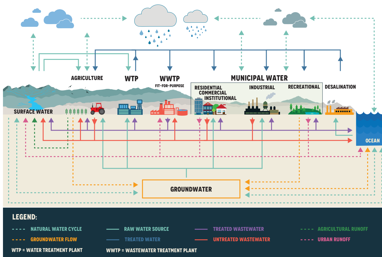
Figure 1.1 Wastewater in the water cycle
